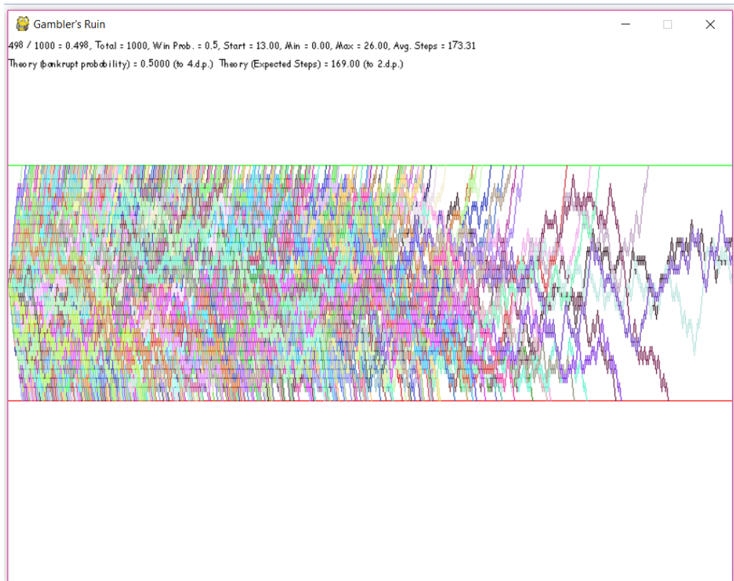
Figure 3: This is a plot of 1000 simulations with k = 13 , p = 0.5 , N = 26 . The theory results in a probability 0.5 of bankruptcy and an expected number of steps of 169. The horizontal green line represents \$N and the horizontal red line represents \$0 . We can see that the simulated probability of 0.498 and the simulated average number of steps of 173 is close to the theoretical values.
