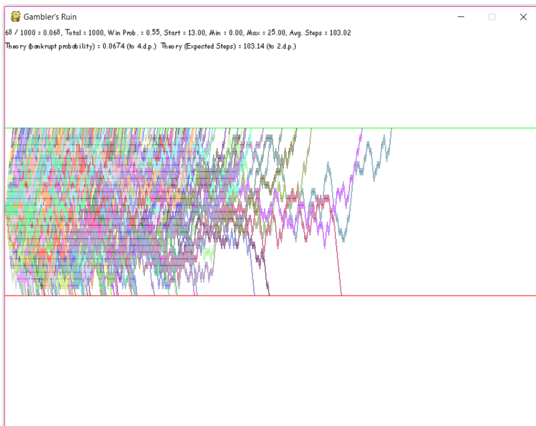
Figure 2: This is a plot of 1000 simulations with k = 13 , p = 0.55 , N = 25 . The theory results in a probability of 0.0674 of bankruptcy and an expected number of steps of 103.14. The horizontal green line represents \$N and the horizontal red line represents \$0 .
